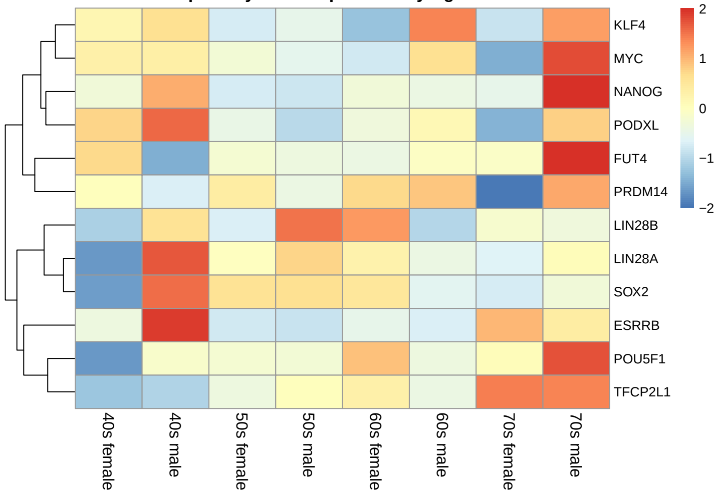
Pluripotency Gene Expression by Age and Sex
