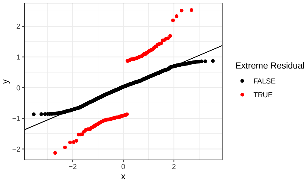
QQ plot of LMM residuals: race
