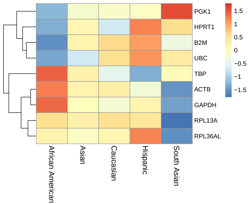
Figure 15: Expression of Housekeeping Genes
