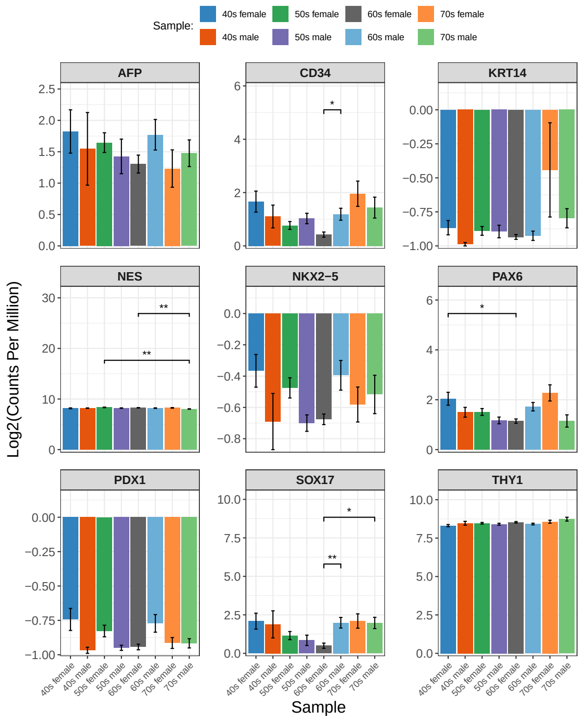
Figure 12: Expression of Differentiation Genes
