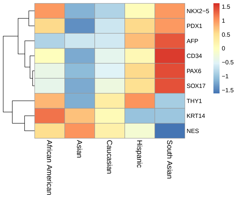
Figure 11: Expression of Differentiation Genes
