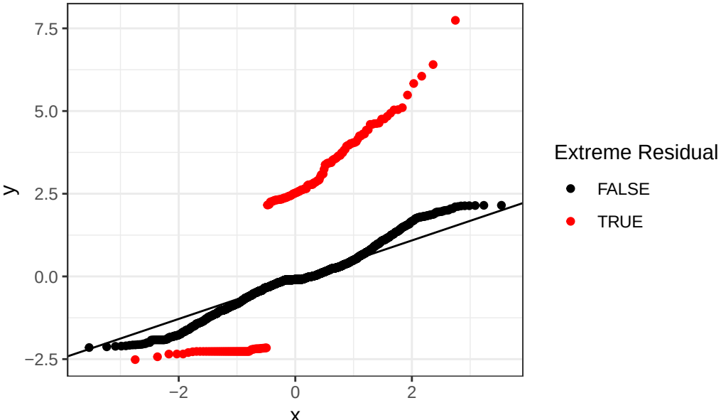
QQ plot of LMM residuals: race
