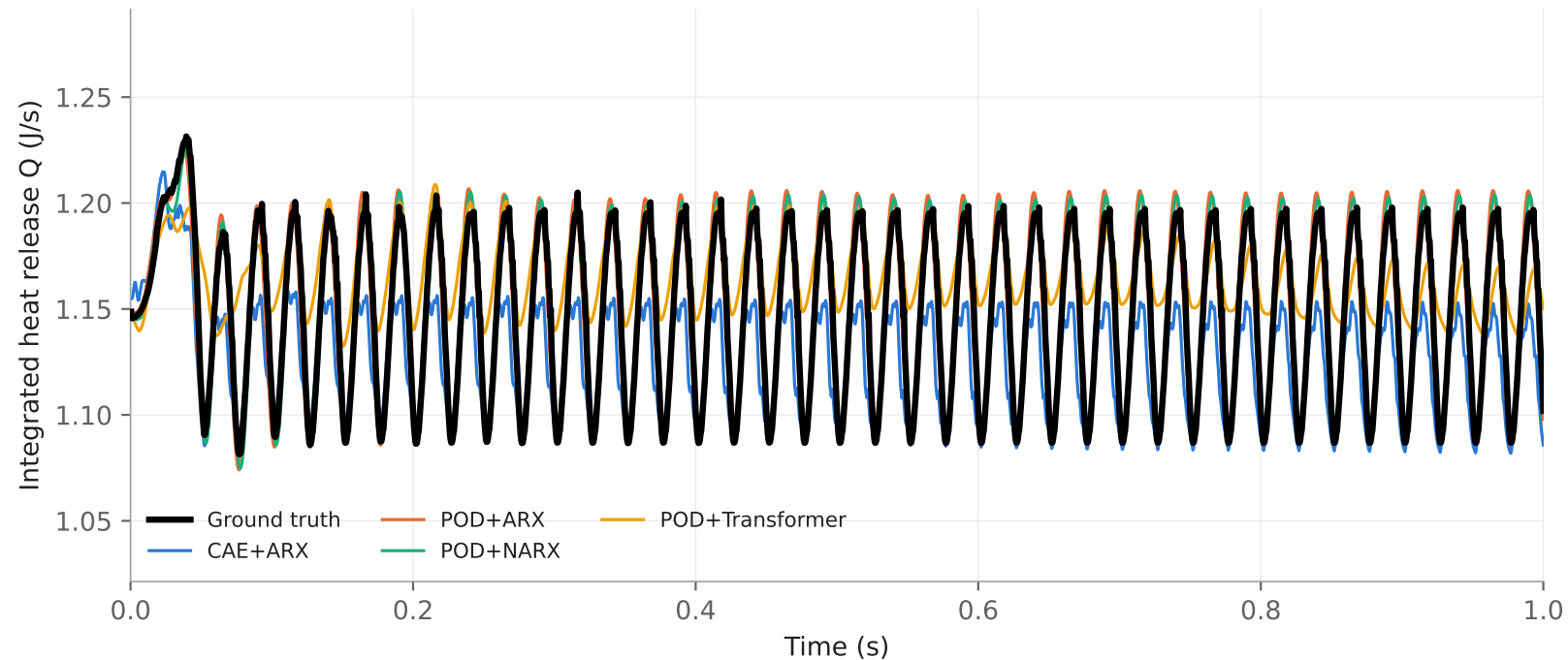
Integrated Q — sine_f40_A03
