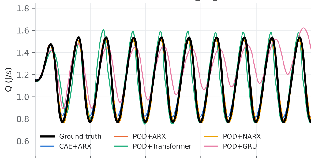
Integrated Q — sine_f40_A03
