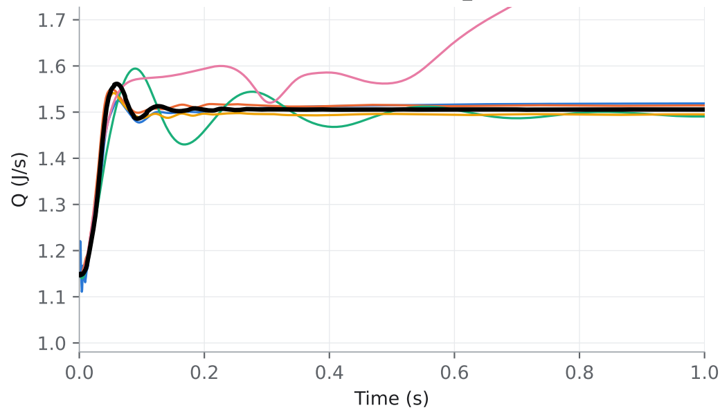
Integrated Q — step_A03
