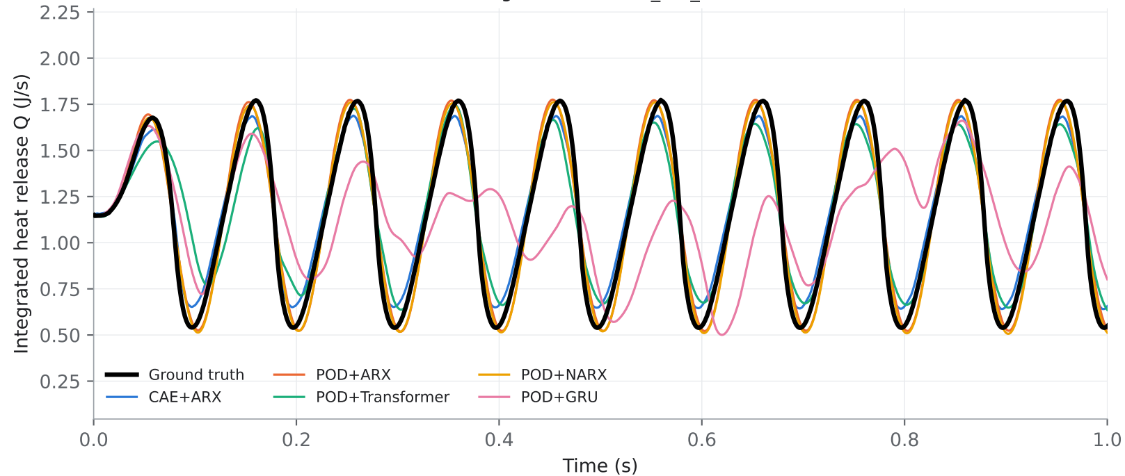
Integrated Q — sine_f10_A05
