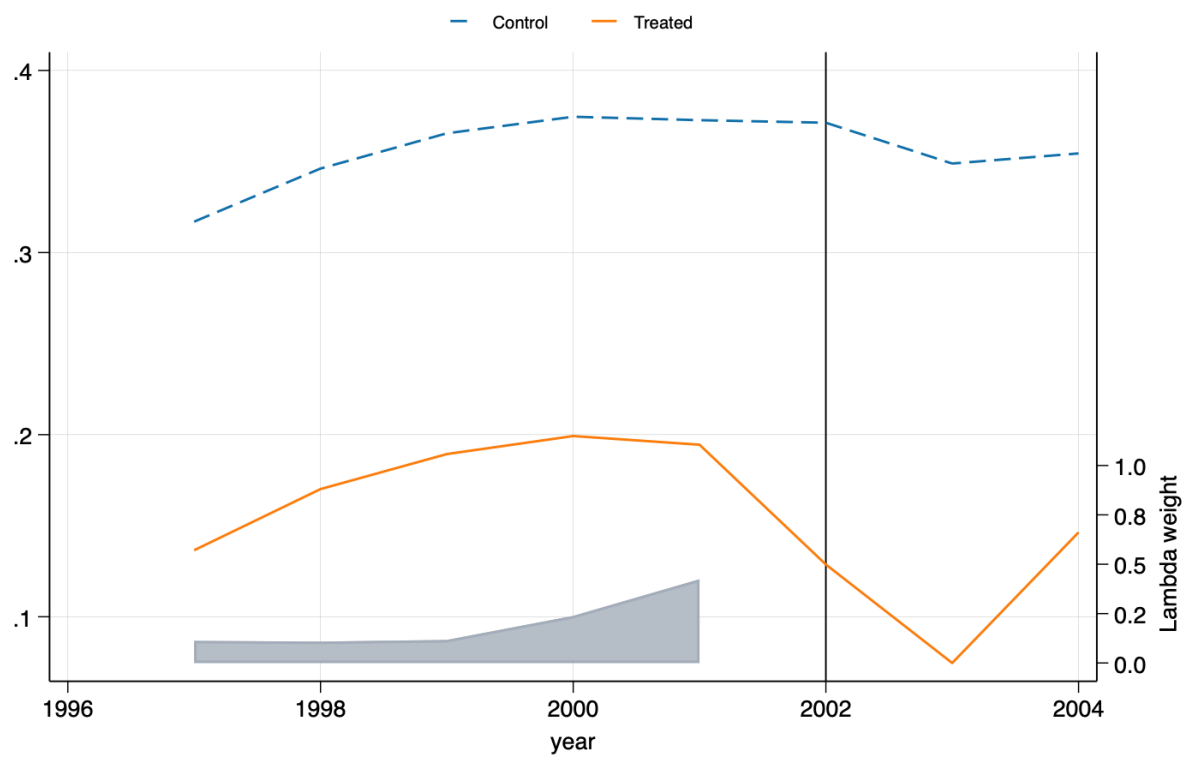
Figure 2: SDID plot
