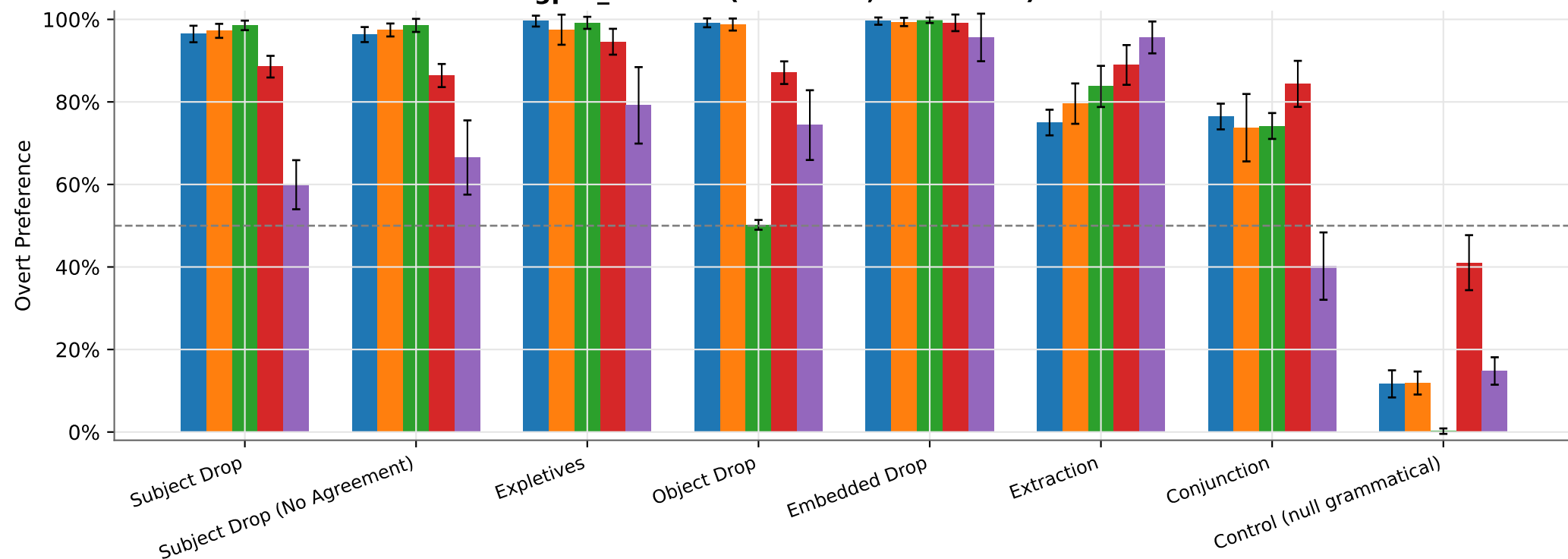
End-State Overt Preference — gpt2_medium (mean±sd, n=10 runs)
