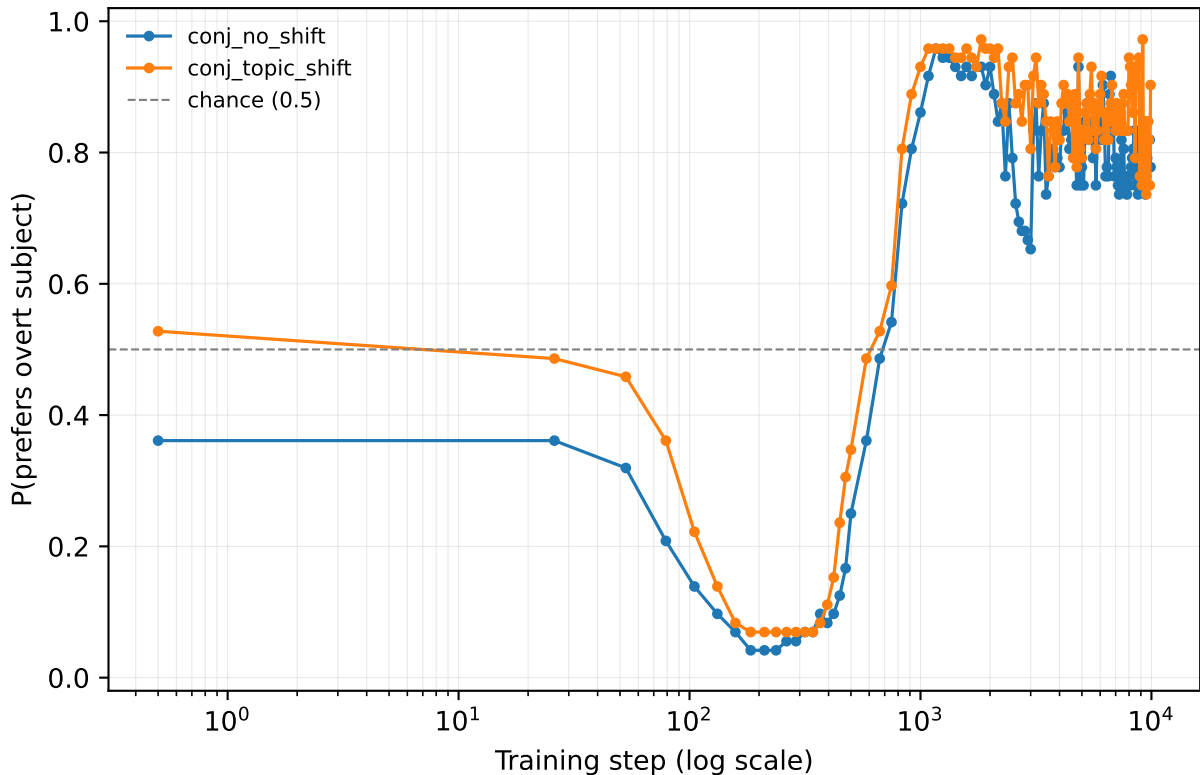
Baseline EN baseline: P(overt) on conjunction trials
