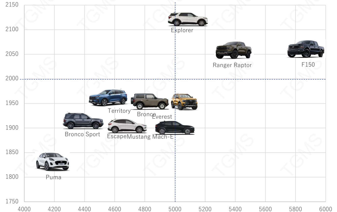
Ford SUVs & Pickups — Overall Length vs. Width
