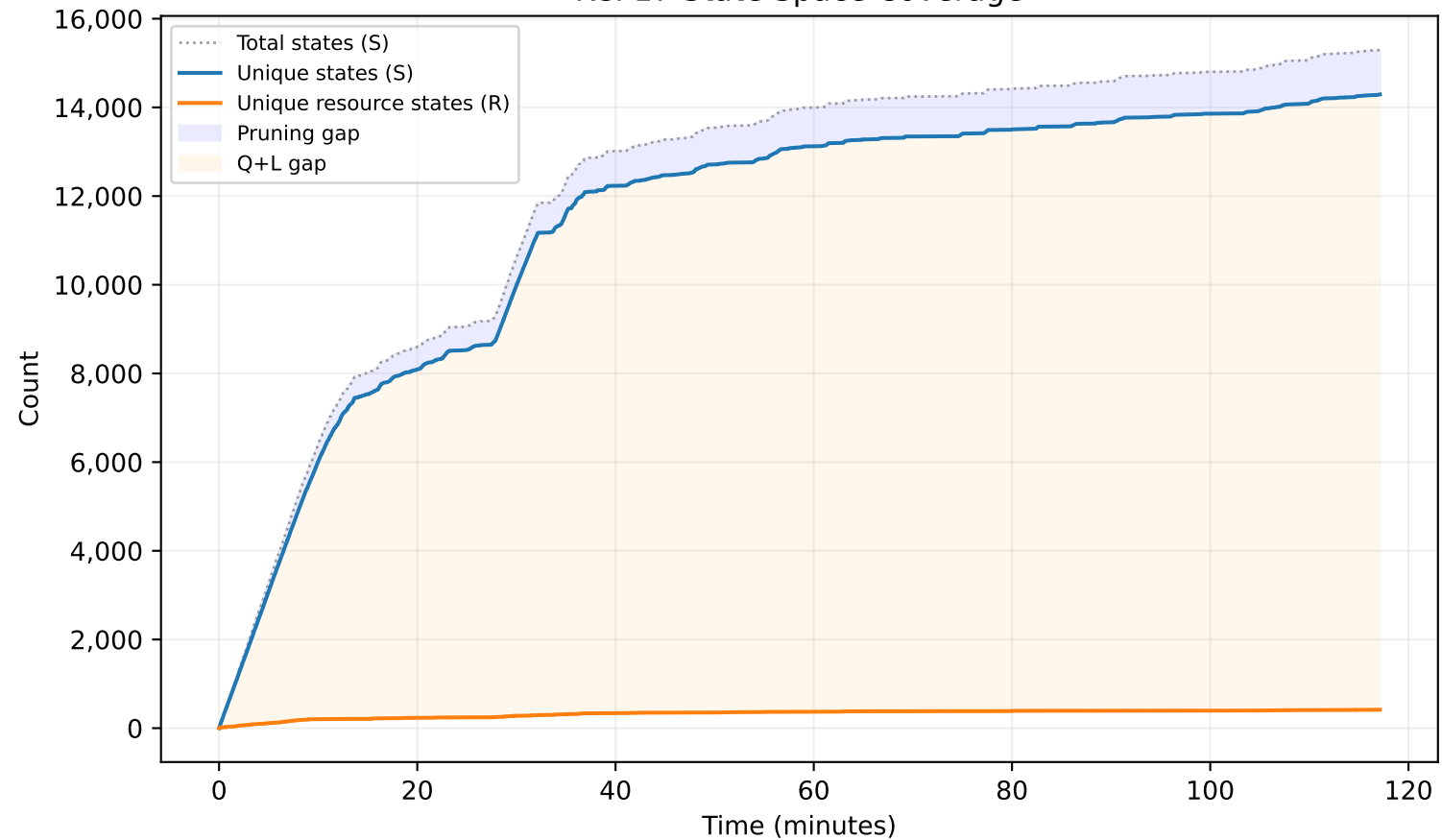
KCP17 State Space Coverage
