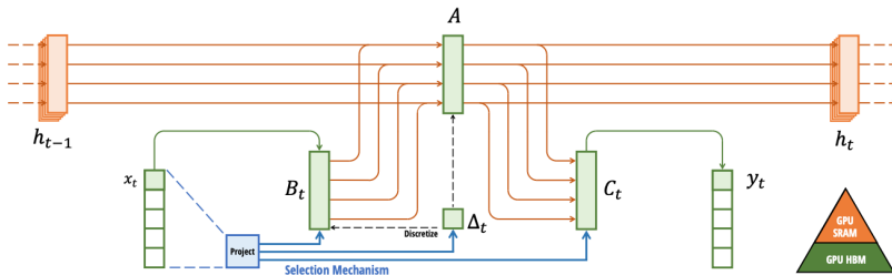
Figure: Selective State Space Model Mechanism.
