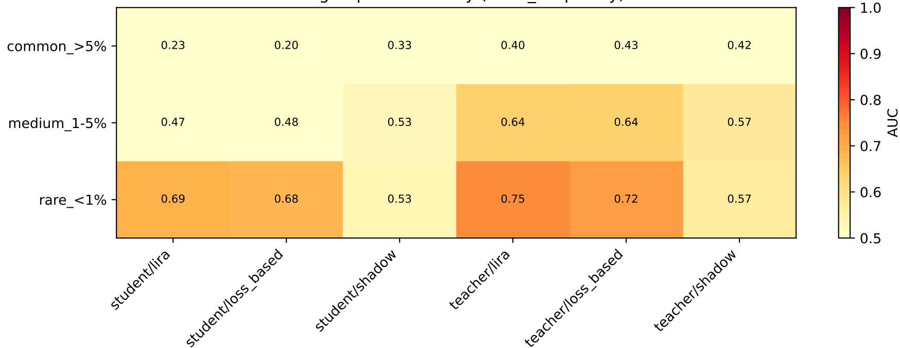
Subgroup Vulnerability (class_frequency)
