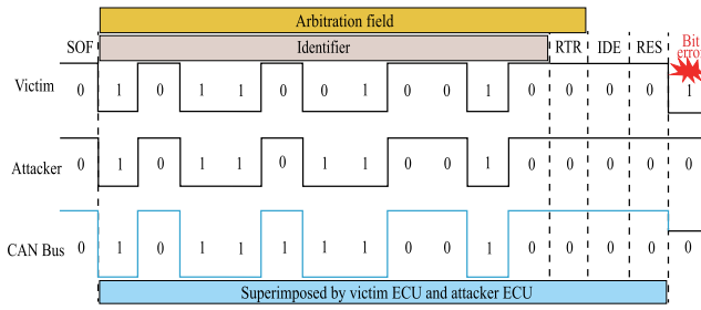
Fig. 3. An example of the bus-off attack.
