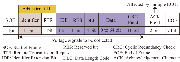
Fig. 2. A standard frame of the CAN bus.
