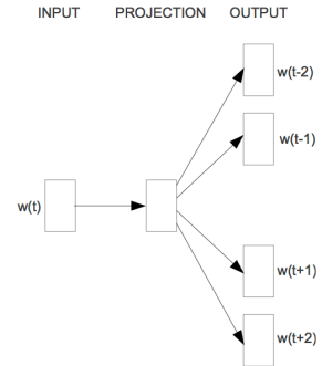
Skip-Gram
