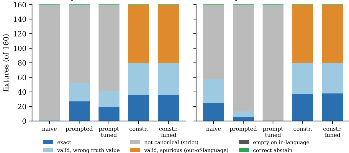
Qwen2.5-0.5B-Instruct
