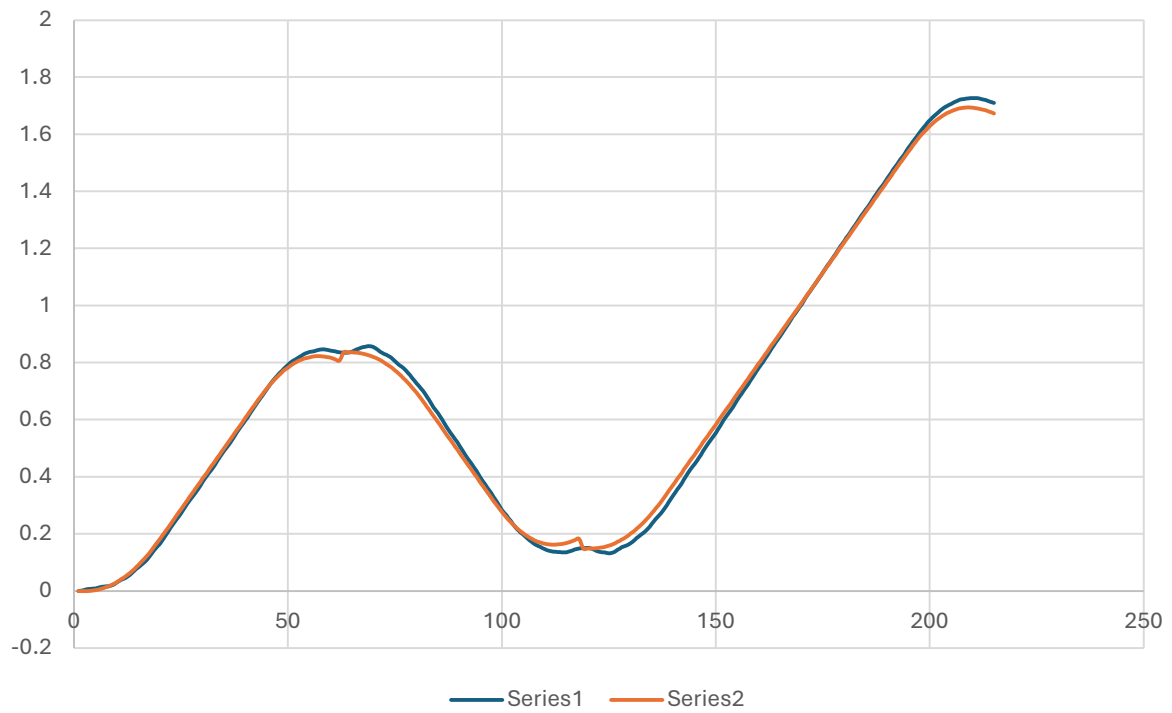
With K_d = 0.2
