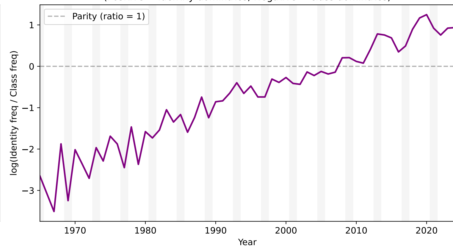
F. Log-Ratio of Absolute Frequencies (Positive = identity dominates; Negative = class dominates)
