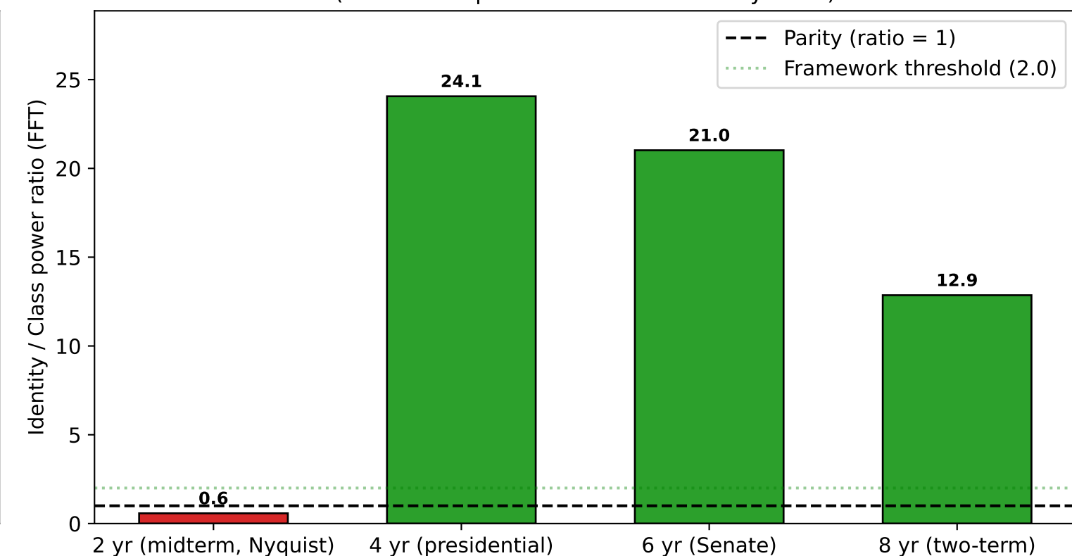
D. FFT Power Ratios at Electoral Cycles (Framework predicts \gg 1 for identity band)
