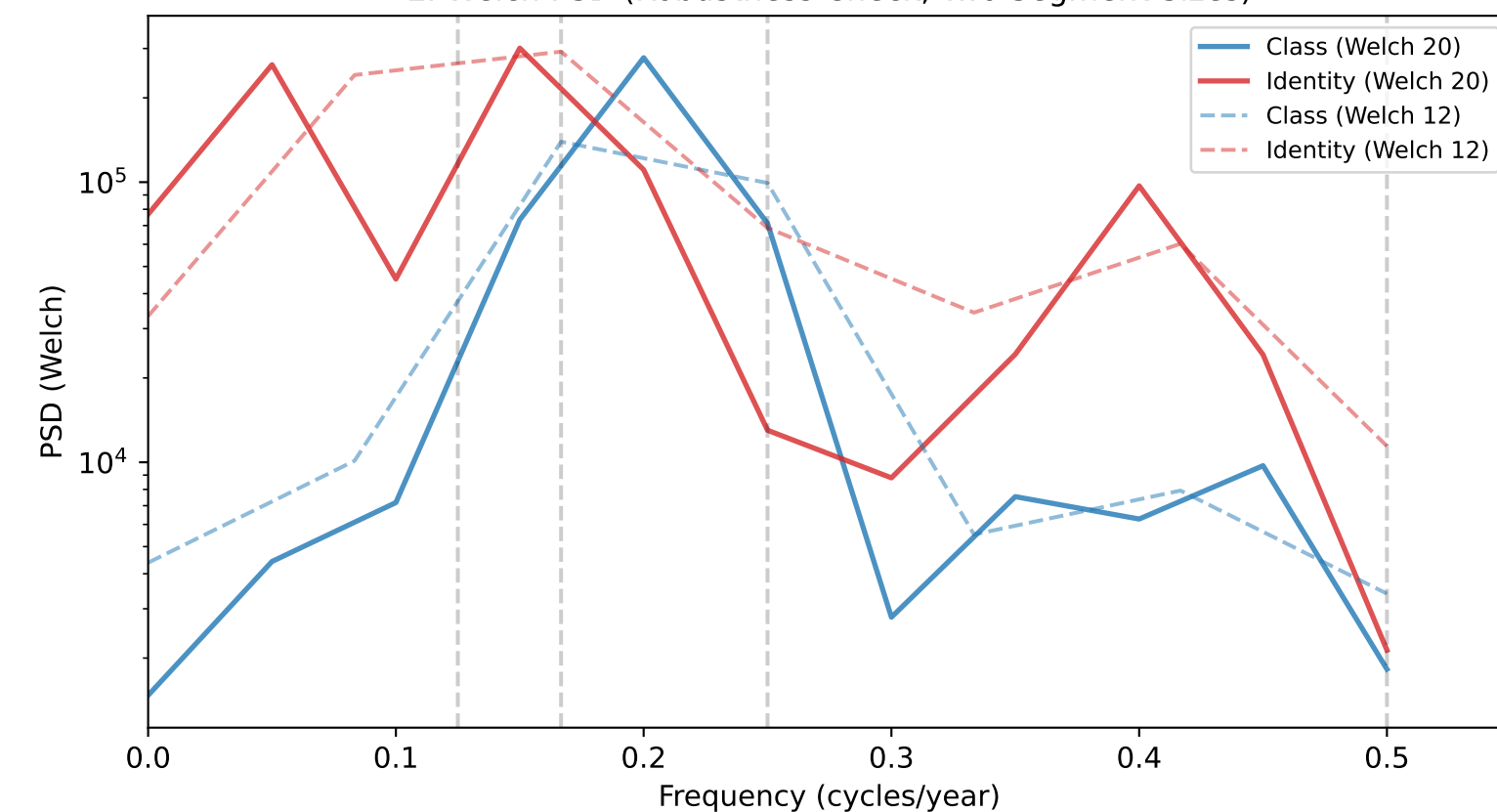
E. Welch PSD (Robustness Check, Two Segment Sizes)
