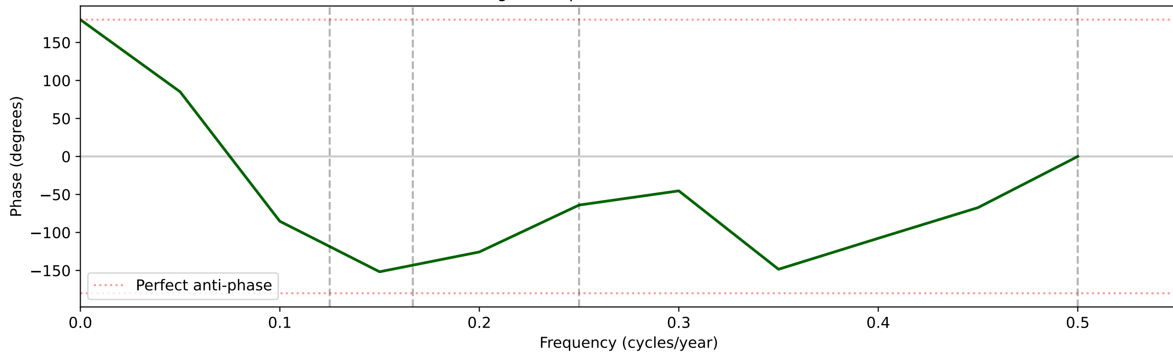
H. Cross-Spectral Phase (+180 deg = anti-phase / destructive interference)
