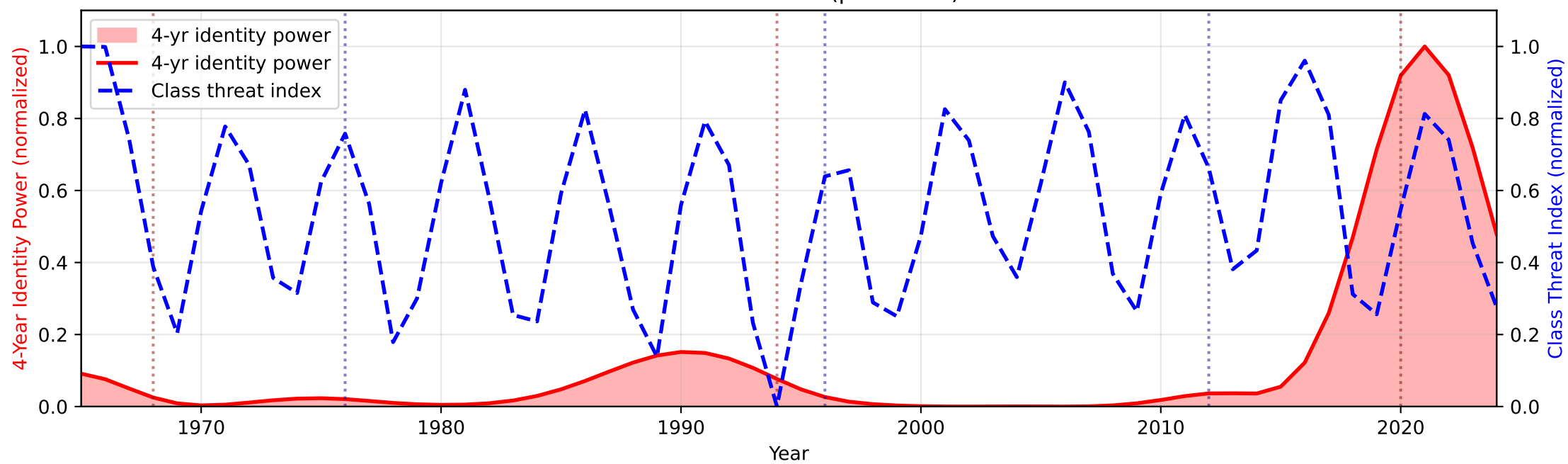
C. 4-Year Carrier Amplitude vs Class-Coherence Threat Pearson r = 0.020 ( p = 0.882 )
