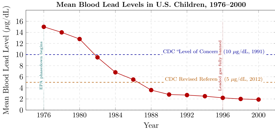
Figure 15.6: The Biological Trajectory of P_{\text{lead}} : Children’s Blood Lead Levels, 1976–2000. Mean blood lead in children aged 1–5 dropped from \sim 15 \mu\text{g}/\text{dL} in 1976 to \sim 1.9 \mu\text{g}/\text{dL} by 2000—an 87% decline directly correlated with the EPA-mandated phaseout. The generation exposed to >10 \mu\text{g}/\text{dL} in the 1960s–1970s reached peak offending age in the late 1980s–early 1990s; the detoxified generation that followed drove the Great Crime Decline. The CDC’s own “Level of Concern” was not set until 1991— after the damage was done. Sources: CDC NHANES II, III, and subsequent cycles.
