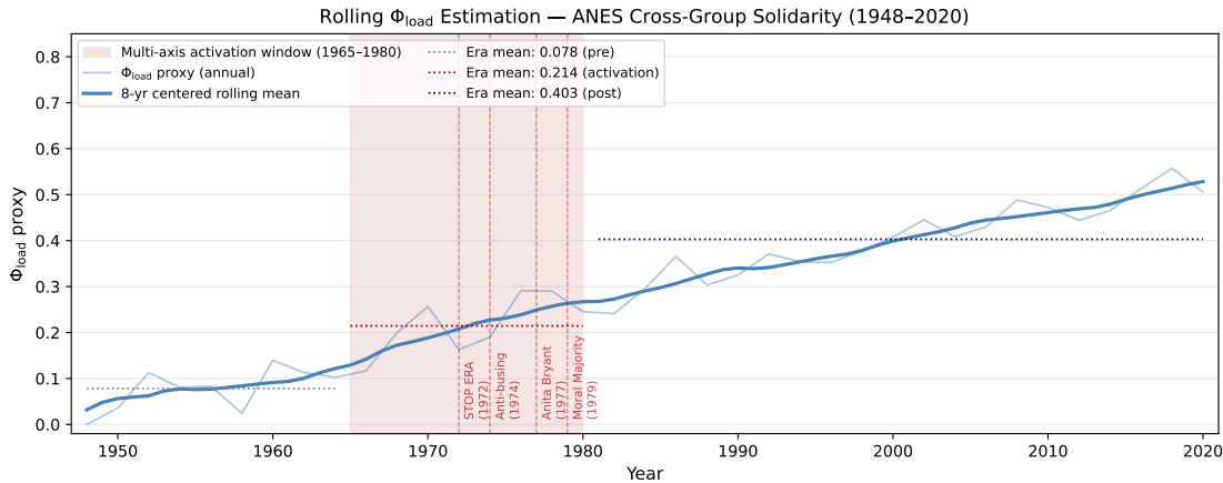
Figure 14.15: Rolling \Phi_{load} Proxy, 1948–2020 (eq:45). The annual proxy ( 1 - \text{cross-group solidarity} / \text{max} ) and its 8-year centered rolling mean are shown with a shaded band for the 1965–1980 multi-axis activation window and vertical markers for four axis-injection events: STOP ERA campaign (1972), anti-busing coalition (1974), Anita Bryant’s Save Our Children campaign (1977), and the Moral Majority (1979). Era means confirm a two-step increase consistent with the interference-engine prediction. Reproducible via Paper/scripts/eq40_45_interference_engine.ipynb .
