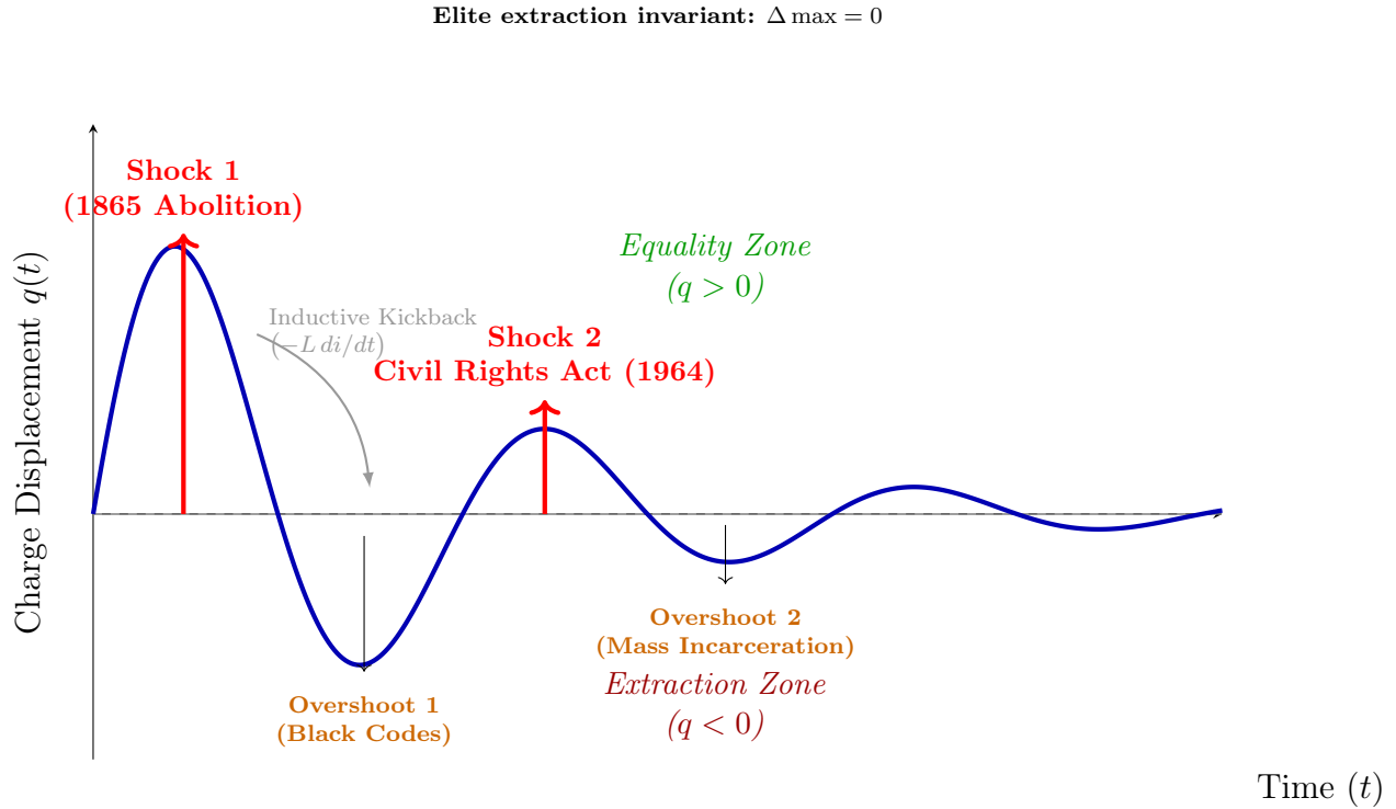
Figure 2.5: Racism as a Damped RLC Circuit (Eq. ??) . Reform shocks inject a driving voltage V_0 that displaces the equality-surplus charge q(t) above the extraction baseline ( q = 0 ). The inductor’s back-EMF ( -L di/dt , inductive kickback) drives the circuit past equilibrium into the extraction zone ( q < 0 ), producing configurations more lethal than the pre-shock state: Convict Leasing after 1865, Mass Incarceration after 1964. Each successive cycle damps faster as \alpha = R/(2L) increases—the system expands its carceral resistance R with each adaptation. Note: The plotted parameters ( Q_0 = 1.6 , \alpha = 0.35 , \omega_d \approx 110 ) are illustrative; they render the two documented shock-and-overshoot cycles legible, not derived from empirical calibration.
