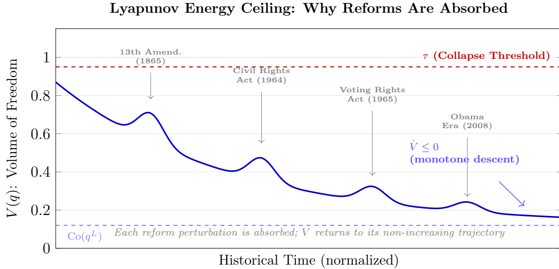
Figure 14.5: The Lyapunov Energy Ceiling. The Lyapunov function V(q) —the “volume of freedom” available to the population—is subject to \dot{V} \leq 0 under the closed-loop dynamics of Equation ???. Each historical reform (13th Amendment, Civil Rights Act, Voting Rights Act, Obama Era) produces a local upward perturbation in V , momentarily expanding the population’s accessible state space. But Theorem ?? guarantees that V returns to a non-increasing trajectory after every perturbation: the control law absorbs each reform and continues driving the population toward the containment set \text{Co}(q^L) . The collapse threshold \tau (dashed red) is never breached. This is the Reform Paradox stated as a stability theorem: the system is Lyapunov stable toward the Elite’s desired configuration. Only structural topological change—severing the spanning tree itself—can alter the descent direction.
