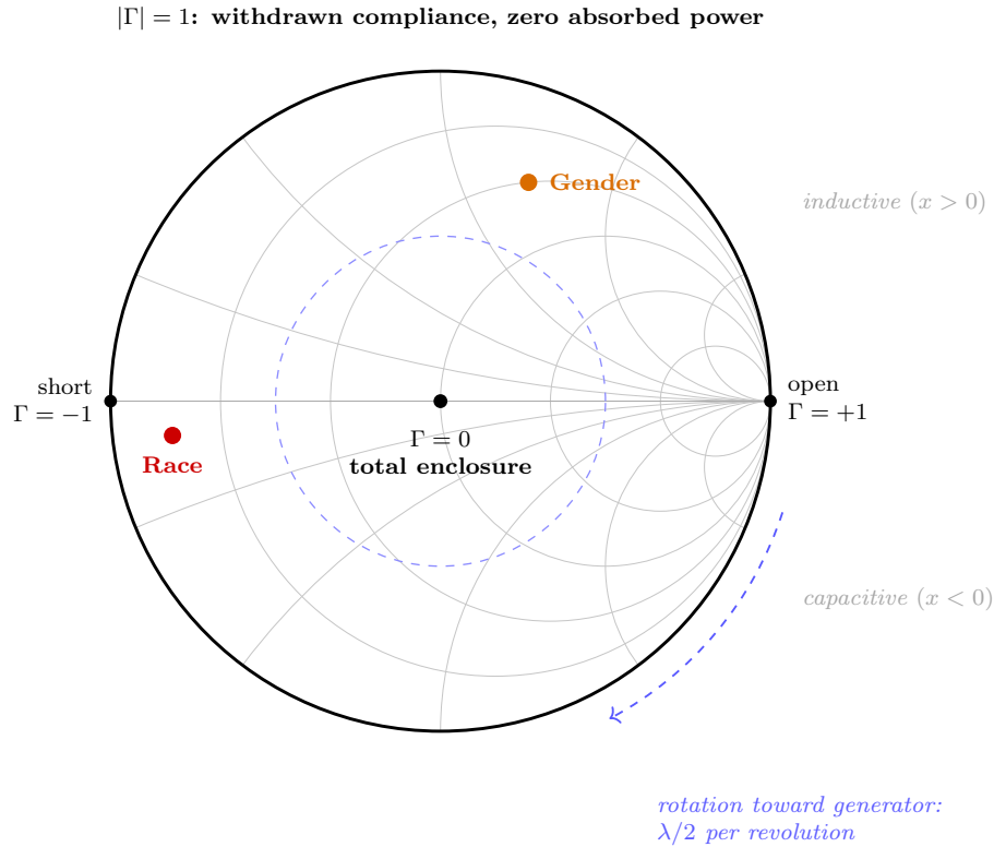
Figure H.1: The Extraction Chart. The reflection-coefficient plane of the extraction line. Every passive load occupies a point in the unit disk. The center ( \Gamma = 0 , z = 1 ) is a perfect impedance match and corresponds to total enclosure, \mathcal{S}_{\text{enc}} \rightarrow 1.0 , with all incident suppression absorbed and nothing returned. The rim ( |\Gamma| = 1 ) is withdrawn compliance: a purely reactive termination absorbing zero real power. Grey circles are loci of constant normalized resistance r (material wage) and constant normalized reactance x (psychological wage). Displacement along the line rotates a load clockwise about the center at one revolution per \lambda/2 , which places a short circuit at the open-circuit point after \lambda/4 (Theorem H.3). Coloured markers place the race and gender sub-bands using exploratory dominant periods recovered by Lomb–Scargle from the selected SCOTUS corpus. Sexuality has no resolved period and is unplots. Equation H.14 sets the reactive component using an illustrative Q_k = 3 , which carries Tier 3 status.
