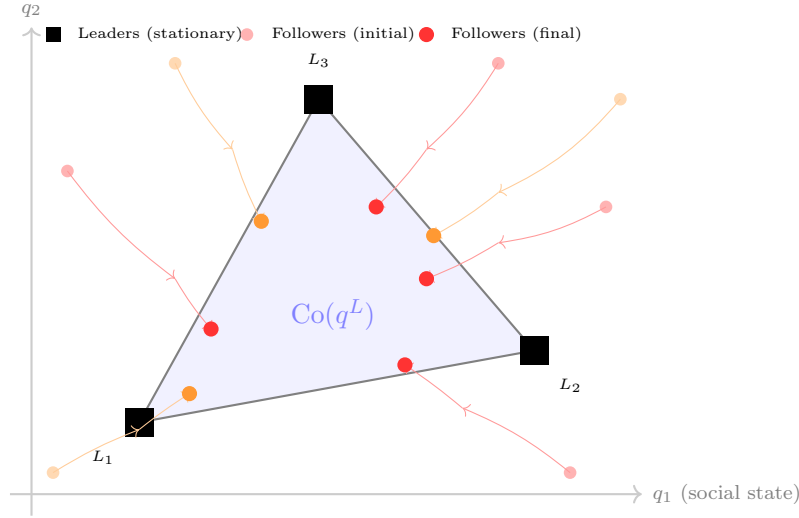
Figure 13.7: Zachary’s Karate Club: A Social Microcosm. Simulation of the fractional-order containment law (Equations ??–??) on a directed subgraph of Zachary’s Karate Club network zachary1977 ; kan_containment . Three stationary leaders ( L_1, L_2, L_3 , black squares) define the convex hull (shaded triangle). Seven followers start at scattered initial positions (light circles) and converge along their trajectories (arrows) to final positions (dark circles) inside the hull. No follower escapes the hull boundary. Structural position in the directed graph—not individual preference—determines the final state. The same theorem that partitions a 10-node karate club is the theorem this book claims partitions 330 million people.
