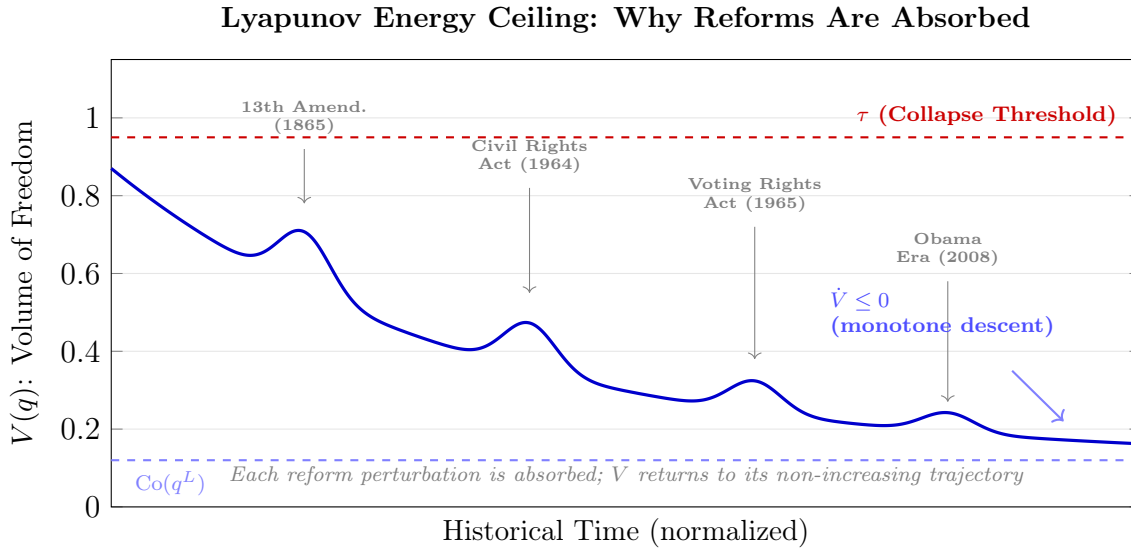
Figure 13.5: The Lyapunov Energy Ceiling. The Lyapunov function V(q) —the “volume of freedom” available to the population—is subject to \dot{V} \leq 0 under the closed-loop dynamics of Equation ???. Each historical reform (13th Amendment, Civil Rights Act, Voting Rights Act, Obama Era) produces a local upward perturbation in V , momentarily expanding the population’s accessible state space. But Theorem ??? guarantees that V returns to a non-increasing trajectory after every perturbation: the control law absorbs each reform and continues driving the population toward the containment set \text{Co}(q^L) . The collapse threshold \tau (dashed red) is never breached. This is the Reform Paradox stated as a stability theorem: the system is Lyapunov stable toward the Elite’s desired configuration. Only structural topological change—severing the spanning tree itself—can alter the descent direction.
