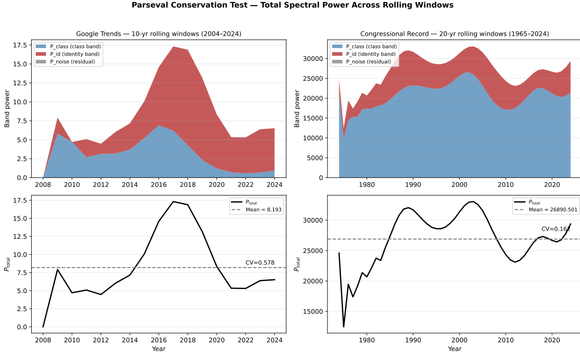
Figure 14.17: Parseval Conservation Test (eq:44). Rolling-window class-band, identity-band, and residual powers are shown stacked (top panels), with total spectral power P_{\text{total}} and its coefficient of variation (bottom panels) for Google Trends (left, 10-yr windows) and the Congressional Record (right, 20-yr windows). The Congressional Record yields \text{CV}(P_{\text{total}}) = 0.162 < 0.30 , supporting approximate Parseval conservation at the institutional layer; the Google Trends \text{CV} = 0.578 exceeds the threshold, indicating that public attention—amplified by social media—is not a closed system, and energy co-spikes (e.g., 2020) are possible. This institutional–attention divergence is itself a theoretically meaningful finding: spectral conservation holds where political expression is institutionally bounded (floor time, legislative agenda) but breaks down in the open market for public attention. Reproducible via Paper/scripts/eq40_45_interference_engine.ipynb .
