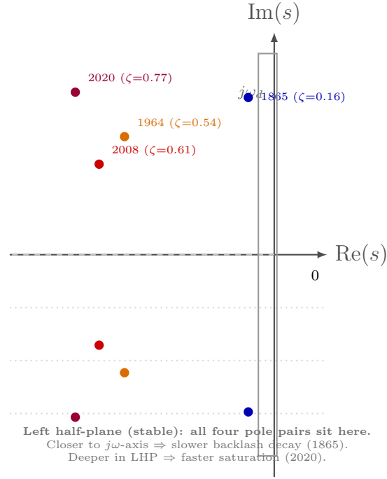
Figure 13.11: Laplace-plane pole plot of the four fitted shock transfer functions. Each pair of complex-conjugate poles s_{\pm} = -\zeta\omega_n \pm j\omega_d is plotted schematically in the left half-plane; horizontal spacing encodes \zeta\omega_n (decay rate), vertical spacing encodes \omega_d (oscillation frequency). Poles migrate leftward and outward over historical time: the engine’s shock response becomes faster and more oscillatory with each successive era. Positions are schematic; exact fitted values are reported in Section 13.1.3 and in Paper/scripts/spectral_laplace.ipynb .
