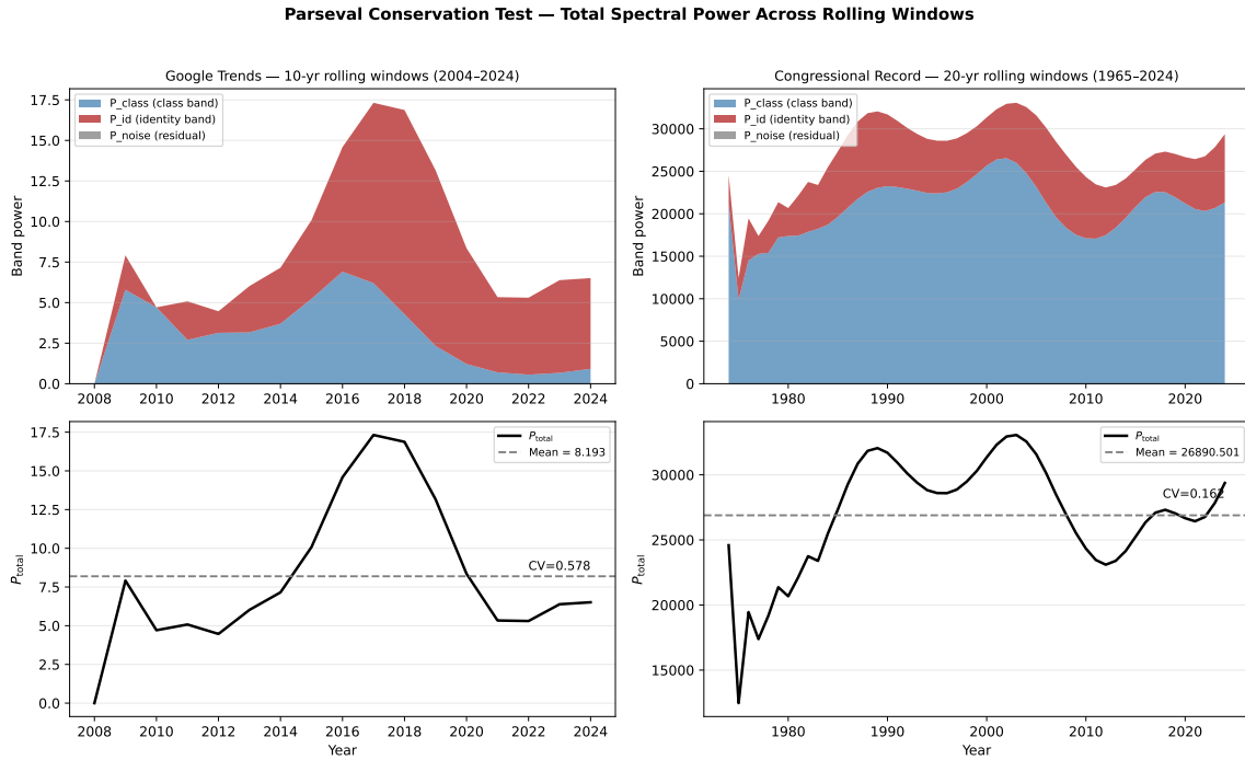
Figure 13.17: Parseval Conservation Test (eq:44). Rolling-window class-band, identity-band, and residual powers are shown stacked (top panels), with total spectral power P_{total} and its coefficient of variation (bottom panels) for Google Trends (left, 10-yr windows) and the Congressional Record (right, 20-yr windows). The Congressional Record yields CV(P_{total}) = 0.162 < 0.30 , supporting approximate Parseval conservation at the institutional layer; the Google Trends CV = 0.578 exceeds the threshold, indicating that public attention—amplified by social media—is not a closed system, and energy co-spikes (e.g., 2020) are possible. This institutional–attention divergence is itself a theoretically meaningful finding: spectral conservation holds where political expression is institutionally bounded (floor time, legislative agenda) but breaks down in the open market for public attention. Reproducible via Paper/scripts/eq40_45_interference_engine.ipynb .
