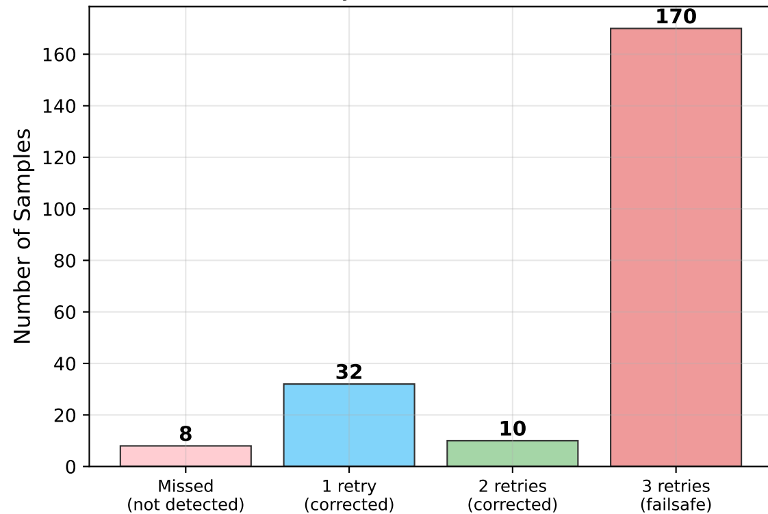
(a) Retry Distribution (N=220)
