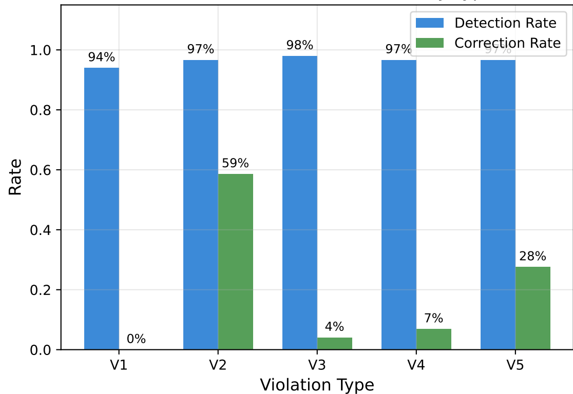
(b) Detection & Correction Rate by Type
