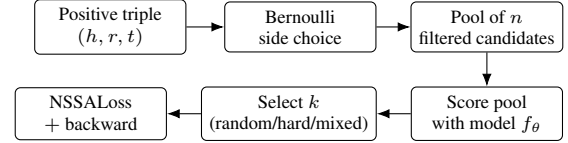
Figure 1. Two-stage negative sampling pipeline. Stage 1 (top): Bernoulli corruption side selection and filtered pool generation. Stage 2 (bottom): model-score-based selection before the loss step.
