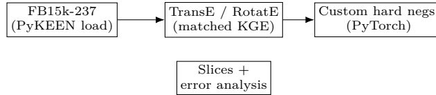
Figure 1: Core pipeline: same filtered evaluation; custom negatives and analysis on the KGE line. GNN (not shown) is optional for later.
