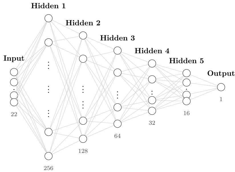
Figure 11: Funnel architecture of the DNN .
