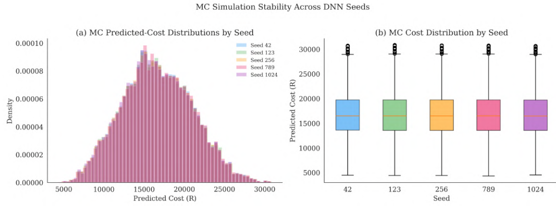
Figure 60: MC predicted-cost distributions across five DNN seeds.
