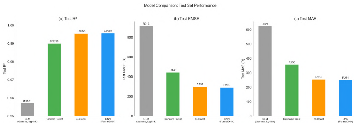
Figure 23: Test-set performance comparison across four model classes.
