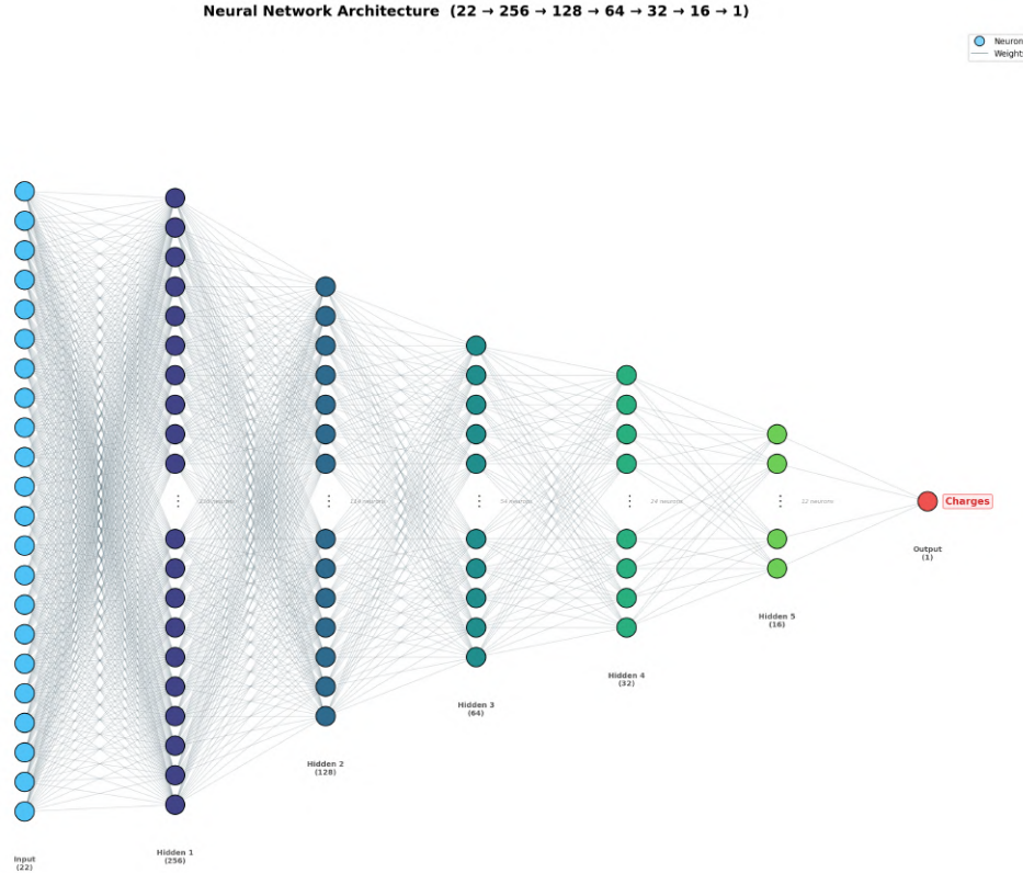
Figure 3: Candidate DNN architecture.
