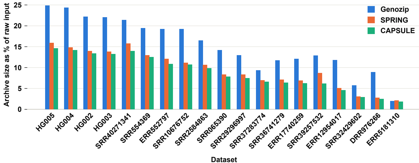
Archive size vs raw input: CAPSULE, SPRING, Genozip
