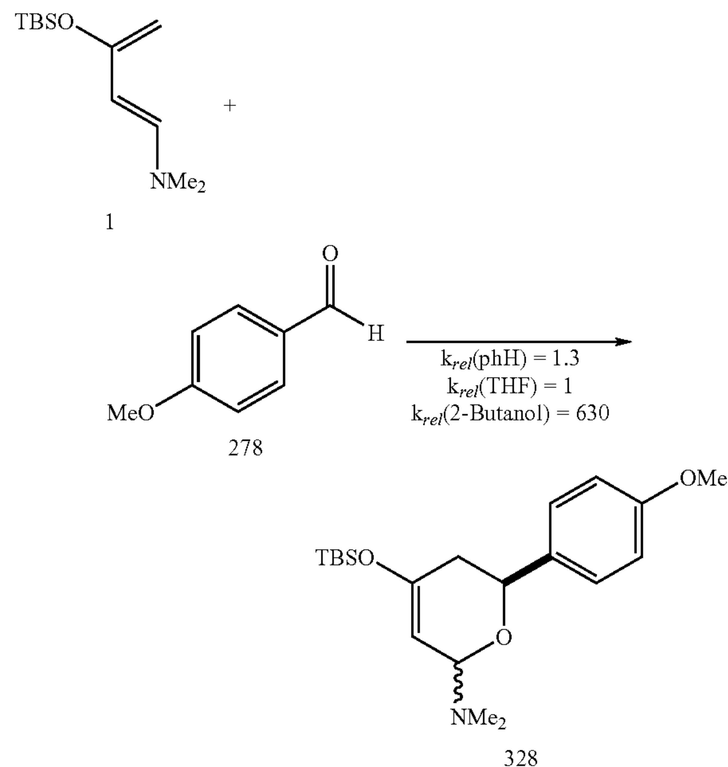
Scheme 8 - Hydrogen Bond Activation by 2-Butanol
