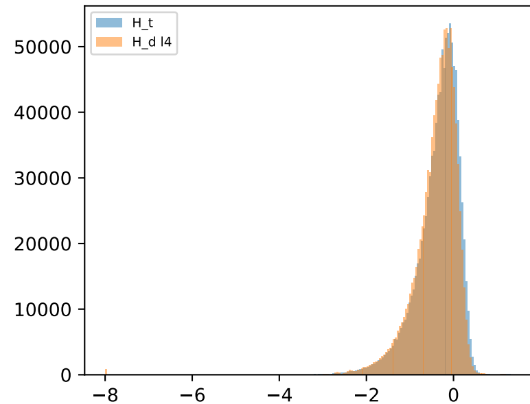
per-token absmax
