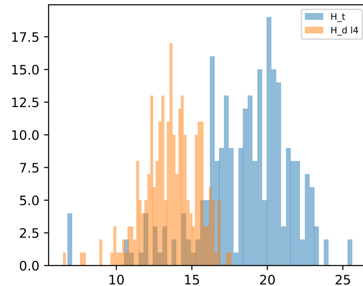
per-token absmax
