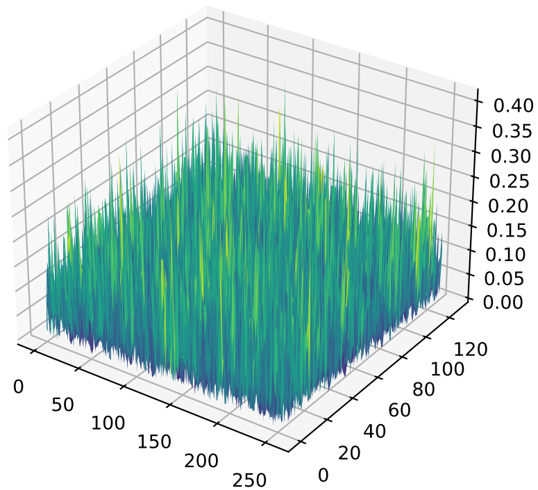
layer0 W_k_proj @ R_C view
