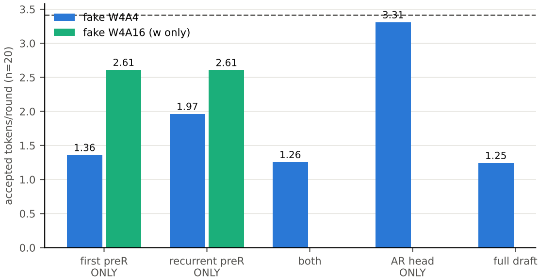
Draft-component quantization (concat-selective; fp16 baseline 3.41)
