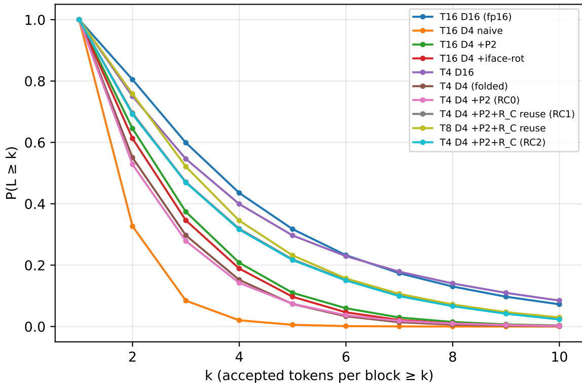
Block-position acceptance survival (MT-Bench, B=10)
