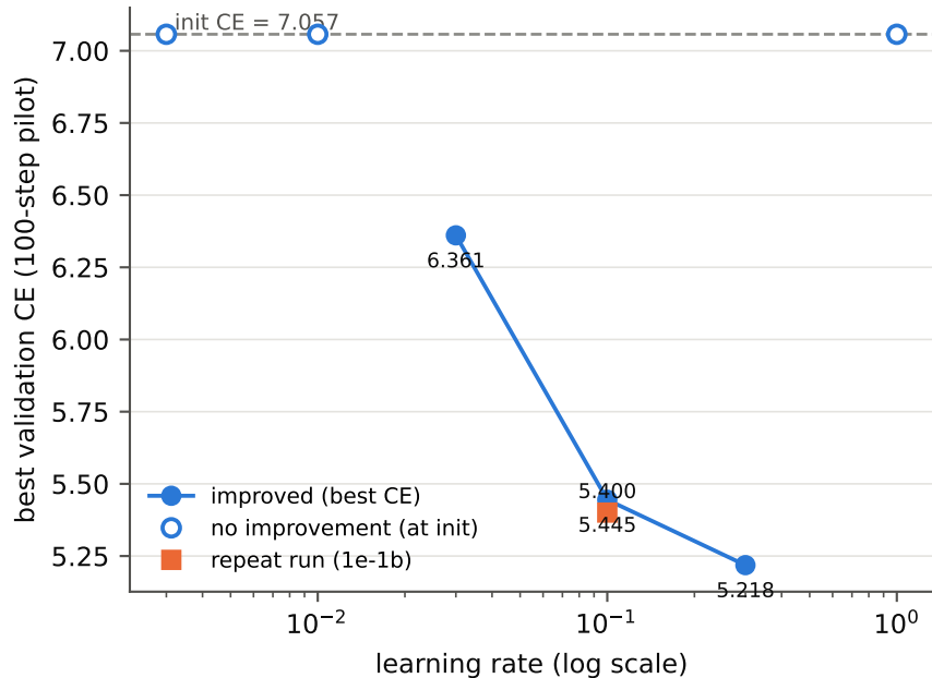
QAT pilot LR sweep (arm Q2)
