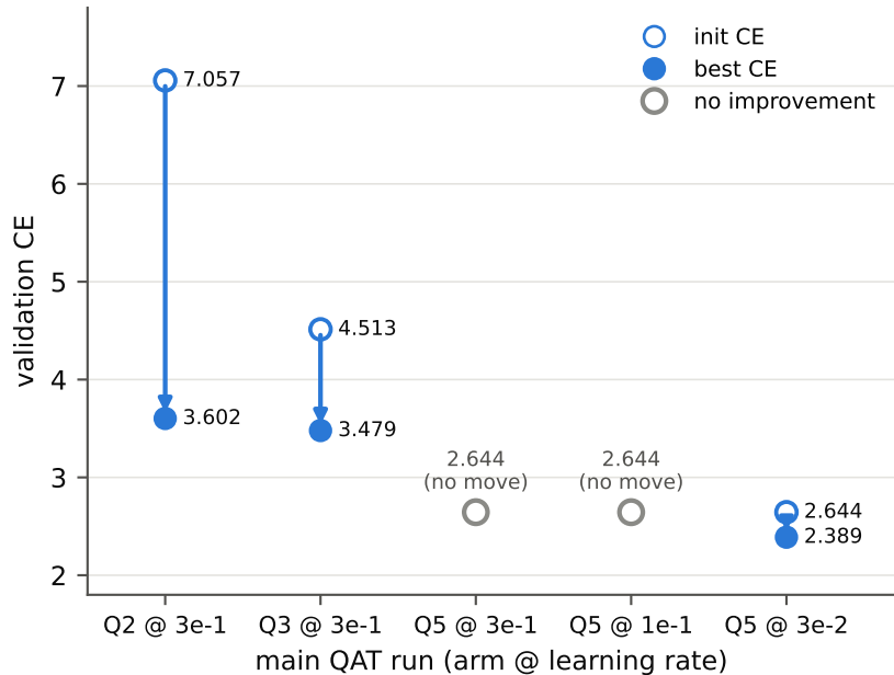
Main QAT runs: init \rightarrow best CE
