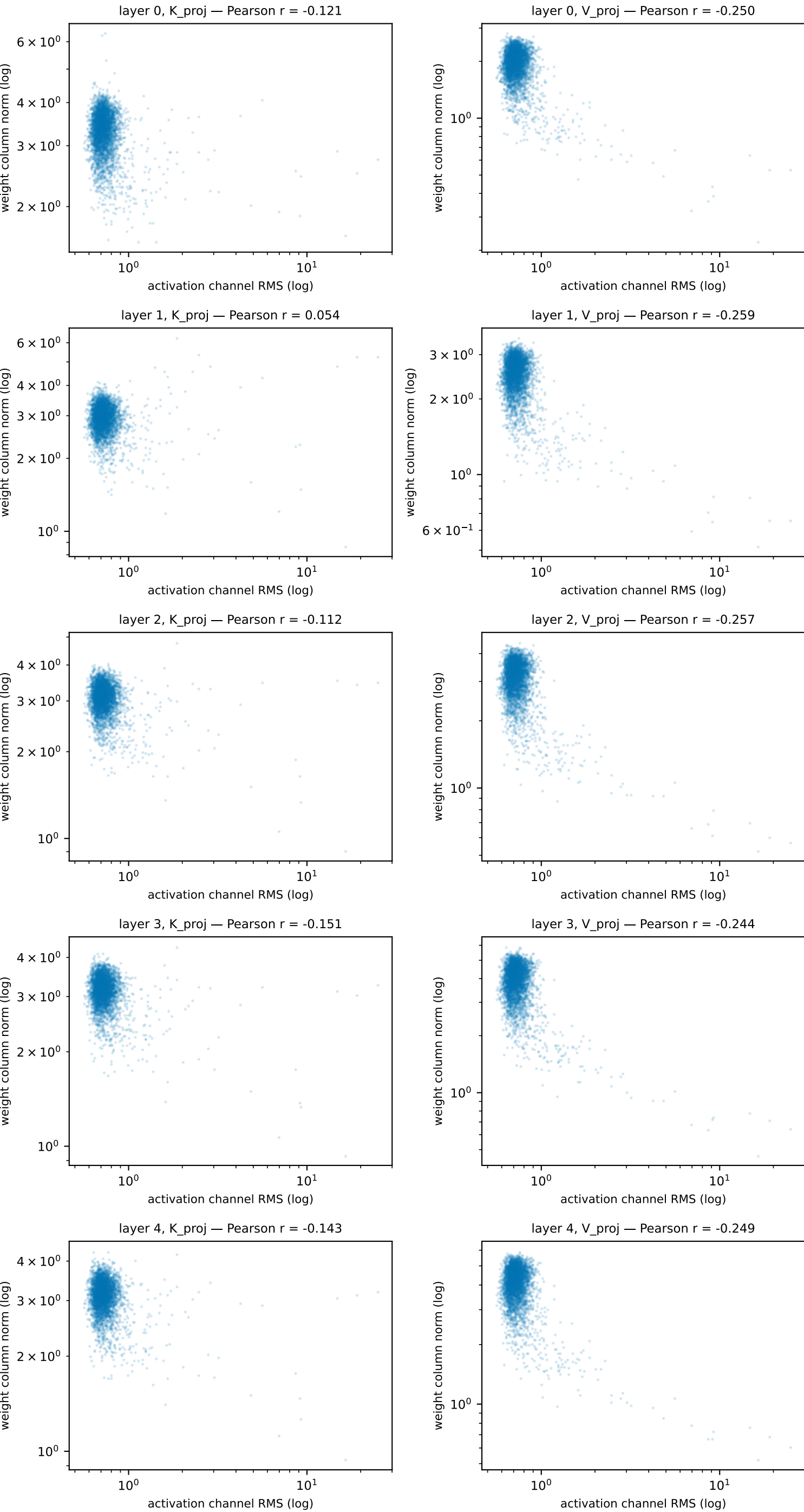
FIG_E activation-vs-weight column alignment, draft ctx K/V projections (per-channel; r computed in raw space)
