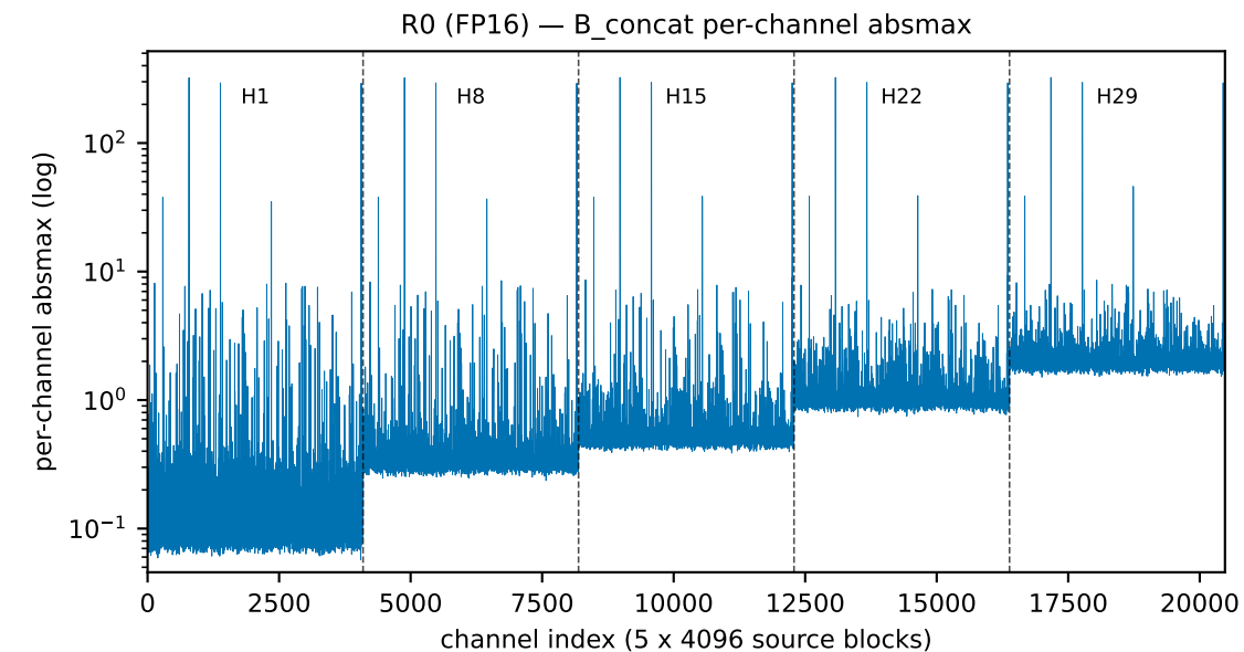
FIG_A target hidden concat B_concat (gsm8k): R0 (FP16) vs R2 (target+draft vanilla-SQ)
