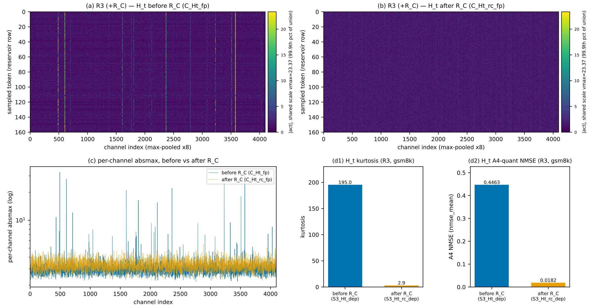
FIG_C H_t before/after context rotation R_C — config R3 (+R_C), gsm8k
