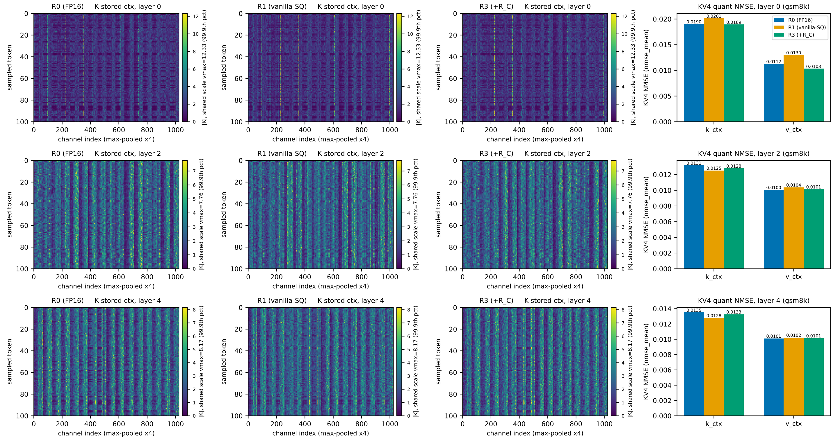
FIG_D stored context-K cache and hypothetical KV4 quantization NMSE — R0 (FP16) vs R1 (vanilla-SQ) vs R3 (+R_C), gsm8k
