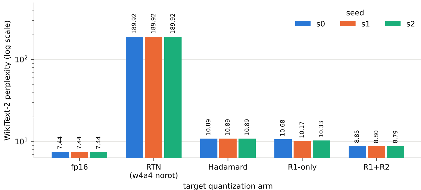
Target W4A4 PPL ladder (Llama-3.1, seeds s0/s1/s2)
