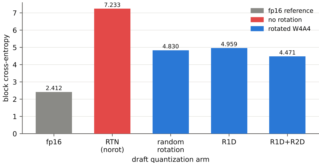
Draft ladder: block CE under W4A4
