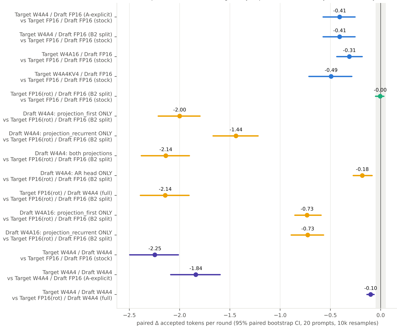
Paired acceptance effects (blue=target-only, aqua=rotation control, yellow=draft-only, violet=both)
