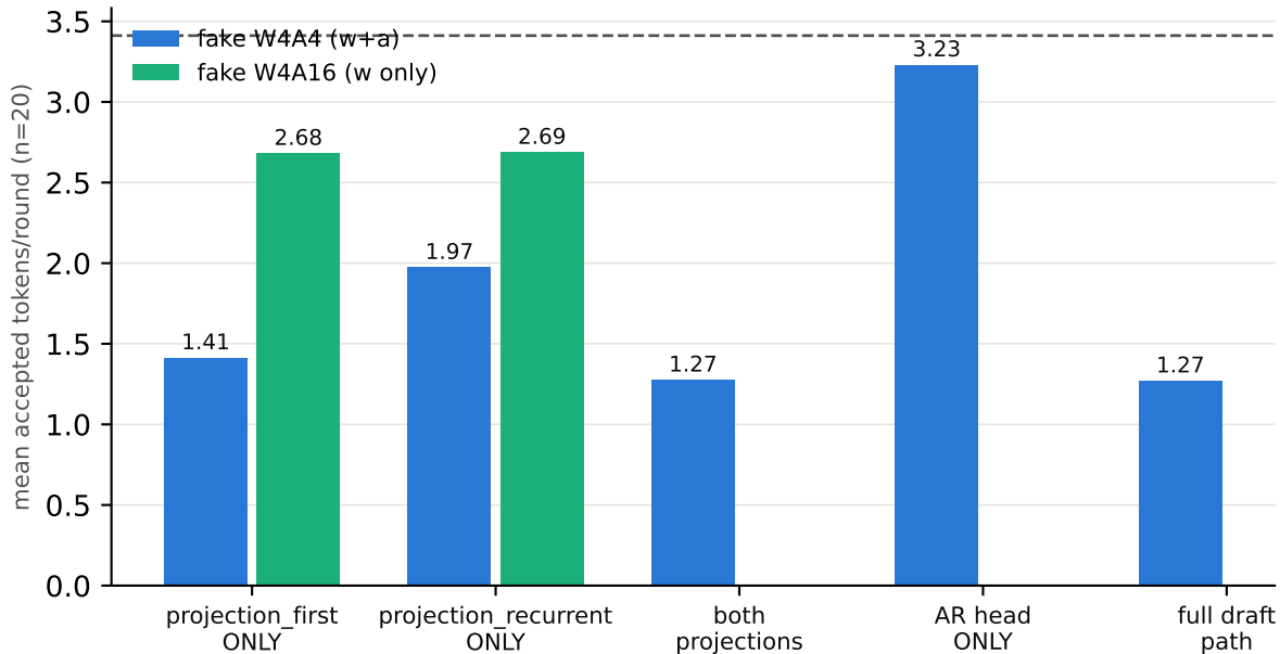
Draft-component quantization ablation (target = rotated FP16; draft embed/head fp16 isolated)
