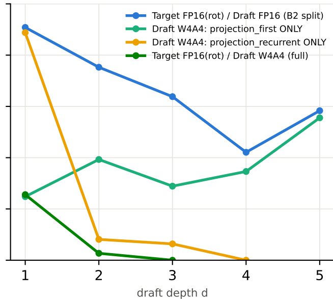
draft-side (target rot-FP16)
