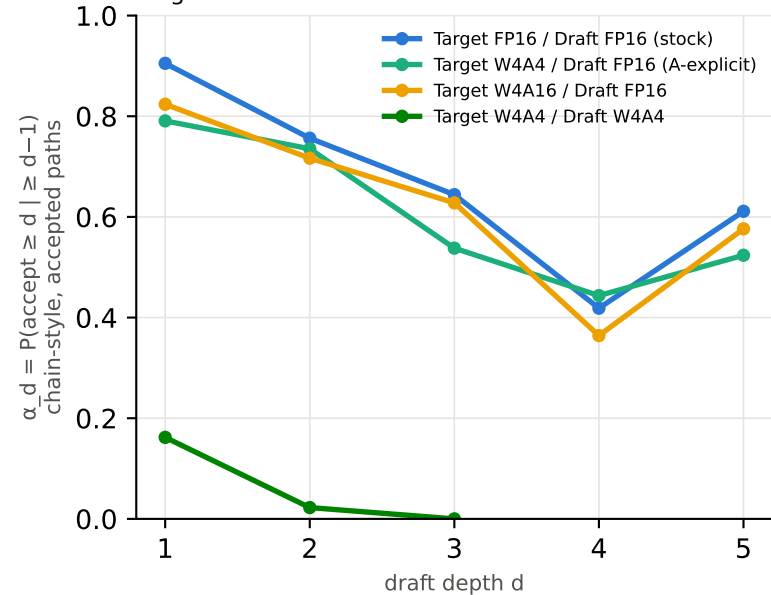
Acceptance by draft depth (greedy, n=20 prompts) target-side
