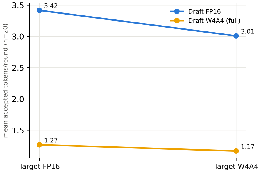
Target \times draft quantization interaction (non-additivity = +0.31)
