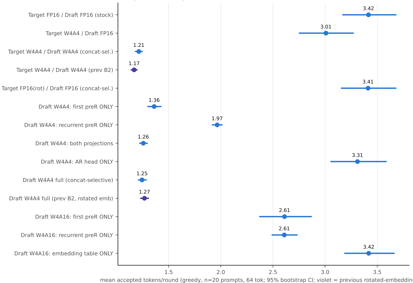
Acceptance across precision combinations and architectures
