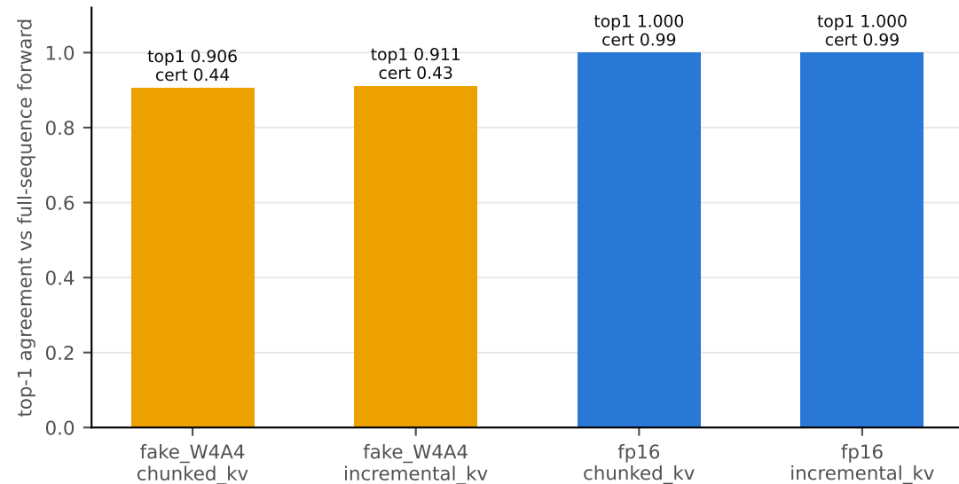
Verifier execution-shape consistency (blue=fp16 target, yellow=fake-W4A4 target; cert = \|\Delta\|_\infty < \text{margin}/2 fraction)
