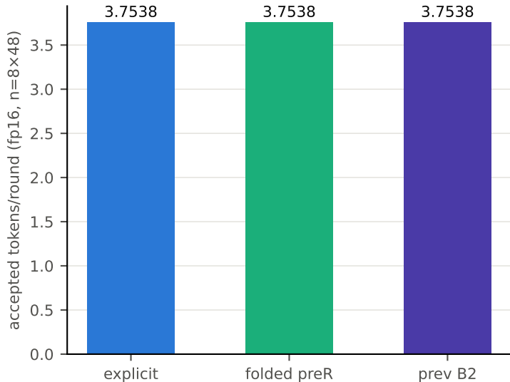
fp16 e2e: all three identical (exact-match 1.0)
